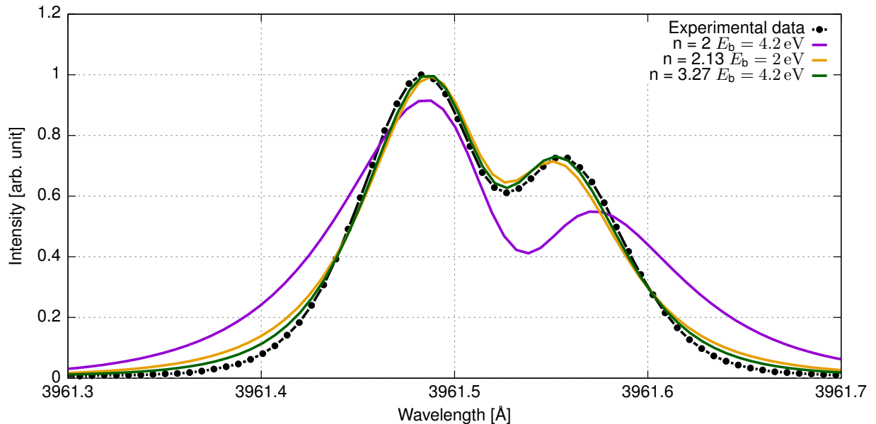
Figure 5. Experimental data at an observation angle perpendicular to the target compared to the model with different parameters: a standard Thompson energy distribution ( n = 2 , E_b = 4.2 eV), with reduced binding energy and a fitted n ( n = 2.13 , E_b = 2 eV) and the most accurate fit ( n = 3.27 , E_b = 4.2 eV).
